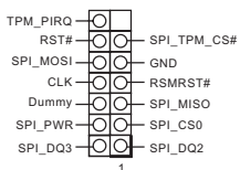
SPI_TPM_J1
